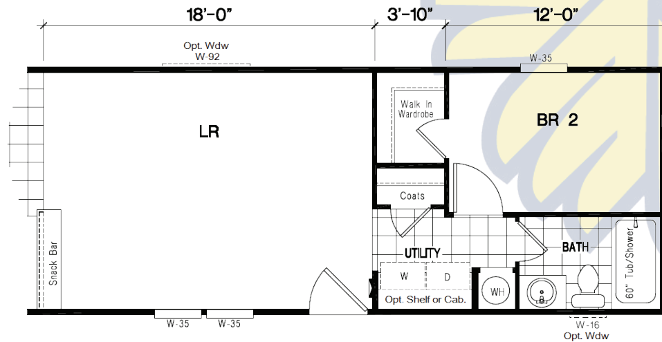
OPTION 2 BEDROOM / ENLARGED LIVING ROOM
